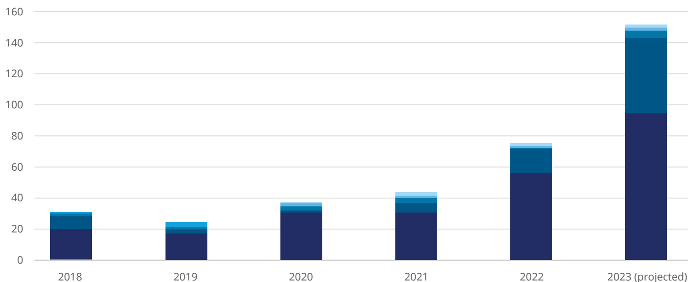
FIGURE 2 | Orbital Launches by US Site: 2018 – 2023
